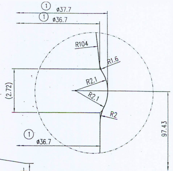
DETAIL 'X' SCALE 10 : 1
