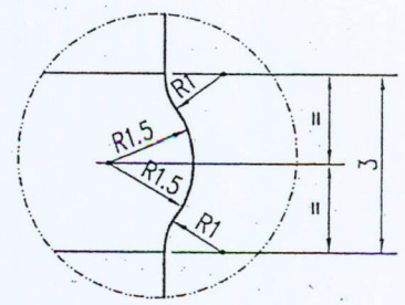
TYPICAL DETAIL 'Y' SCALE 10 : 1
