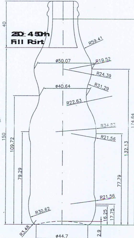
Section view AA Scale 1:1
